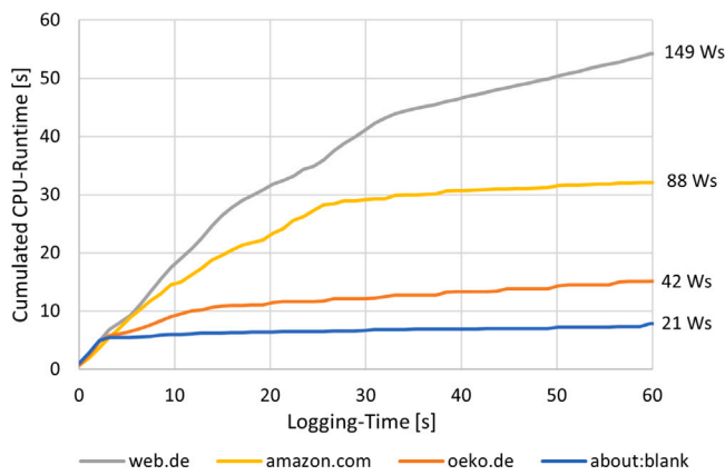
Fig. 8. Cumulated CPU runtime and energy consumption of different website calls (start page).
