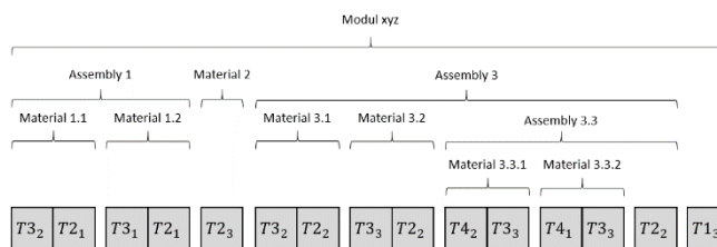
Figure 8. Chromosome-Coding of BOM
