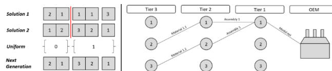
Figure 13. Recombination Point to combine both solutions
