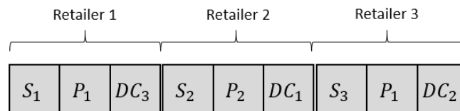
Figure 3. Coding of Chromosomes with Route explanation
