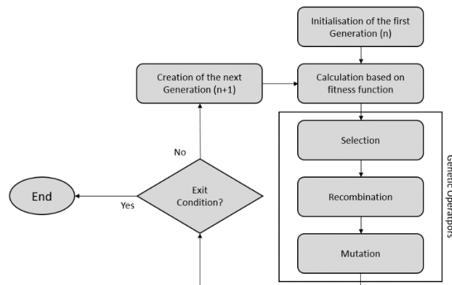
Figure 1. Genetic Algorithm Flow Chart
