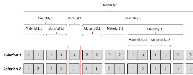
Figure 11. Recombination Point in Chromosomes
