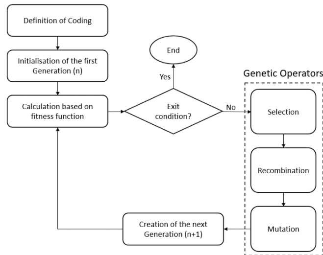
Figure 5. Typical Genetic Algorithm Flow Chart
